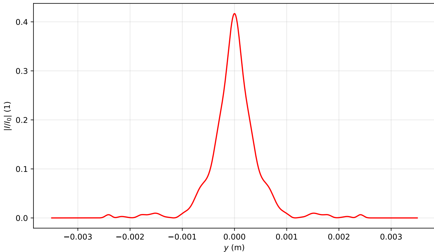
Intensity profile I(x=0, y, z=2.229)/I_0 , P_{in}=4.0P_{cr} , artificial time
